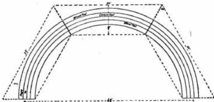
FIG. 44. -- Laying out a curve for electric track.
