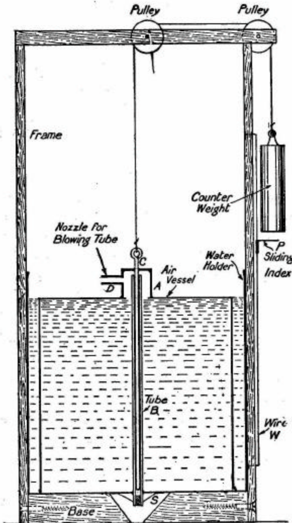
FIG. 166.—Section of lung-capacity tester.
