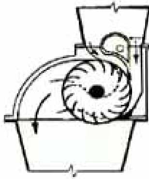
Crossflow Turbine
