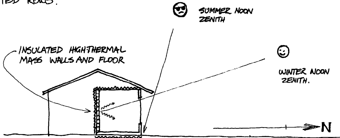
FIG 6:21: SUN/WINDOW/EAVE RELATIONSHIP.
