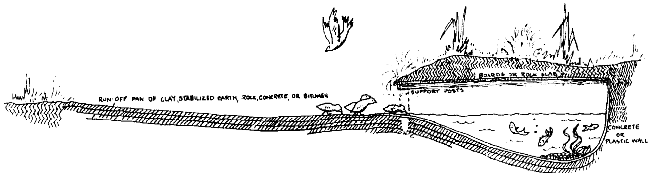
FIG. 5.14: SMALL WELL IN CLAYPAN OR ON ROCK BASE HOLDS WATER FOR QUAIL, PIGEON, LIZARD SPECIES, BEES. FISH AND MUSSELS KEEP WATER CLEAR. CATTLE CANNOT FOUL SUCH WELLS.
