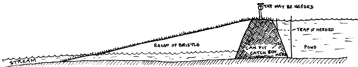
A SLOPE OF NYLON BRUSH BRISTLE, OR TURF, OR ROUGH STONE FOR WRIGGLING .B AND CREEPING SPECIES SUCH AS ELMERS, YABBIES, SHRIMPS, ETC (AFTER MODEL AT LIMERICK, IRELAND).
